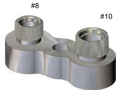
GM Style Horizontal Flat Face Compressor Block BILLET MACHINED , #8 - 3/4"-16 Thrd,& #10-7/8"-14
