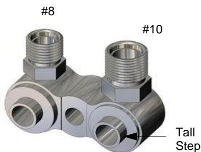
GMLS1 Style Vertical Compressor Block 3/ #8 - 3/4" - 16 Thread & #10 - 7/8" - 14 Thread
