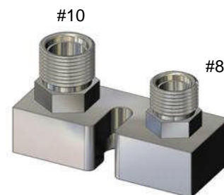
Ford Style Compressor Block W/ #8 - 3/4" - 16 Thread & #10 - 7/8" - 14 Thread
