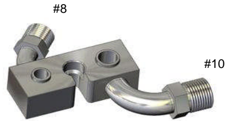
Ford Style FS10 Compressor Block #8 - 3/4" - 16 Thread & #10 - 7/8" - 14 Thread
